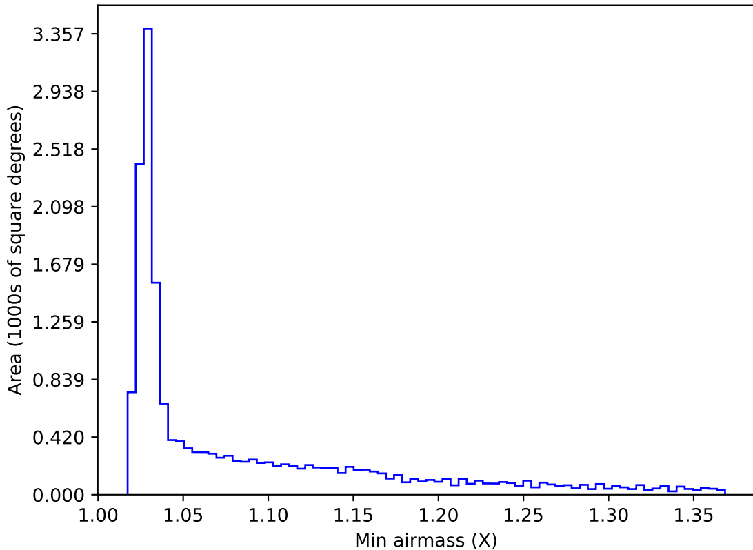
extra_ss_neo7_v3.4_10yrs WFD i band: Min airmass
