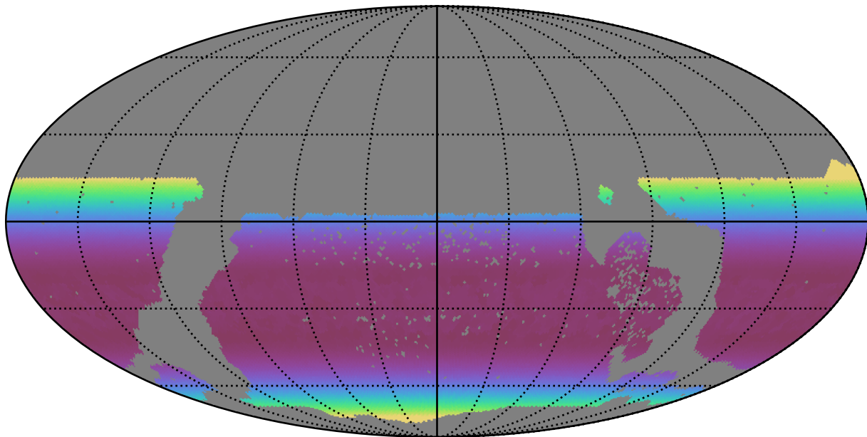
extra_ss_neo7_v3.4_10yrs WFD all bands: Min airmass
