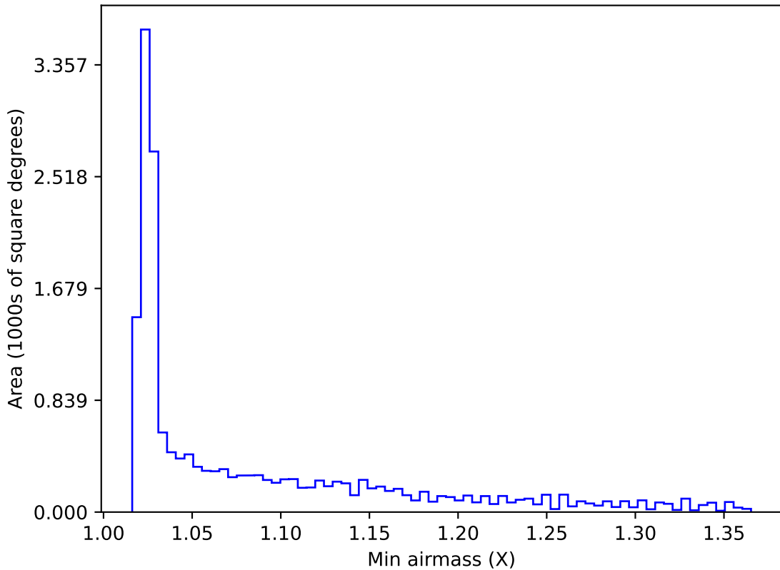
extra_ss_neo7_v3.4_10yrs WFD all bands: Min airmass
