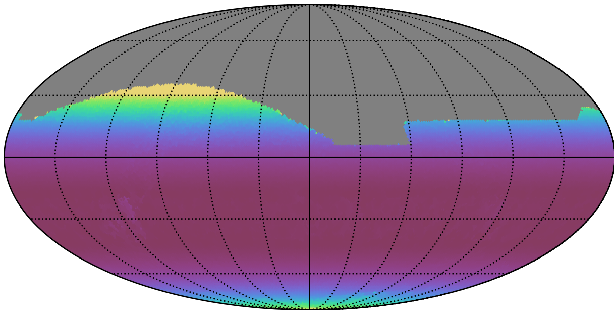
extra_ss_neo7_v3.4_10yrs All sky z band: Min airmass
