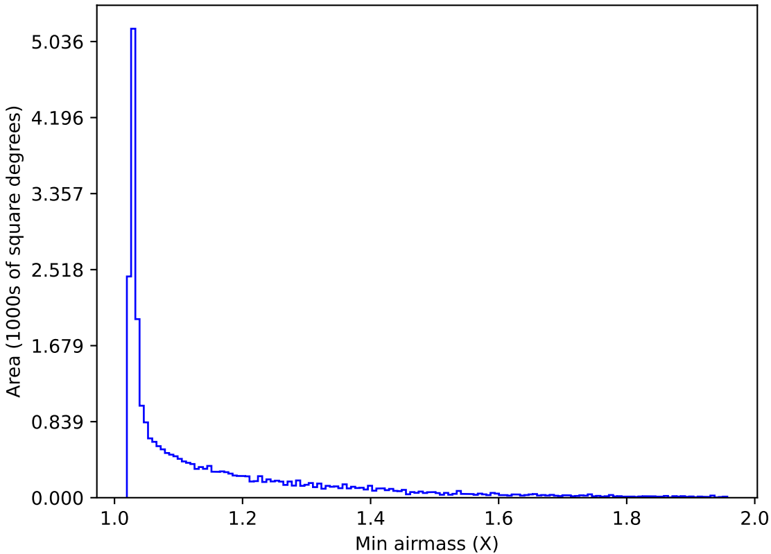
extra_ss_neo7_v3.4_10yrs All sky z band: Min airmass
