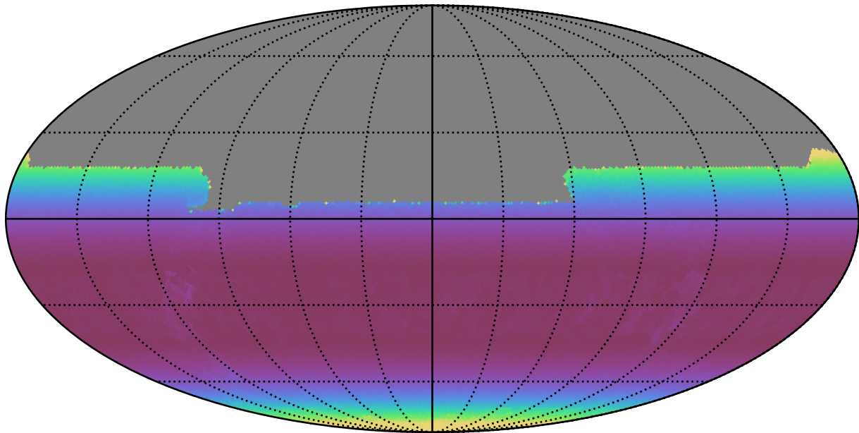
extra_ss_neo7_v3.4_10yrs All sky y band: Min airmass
