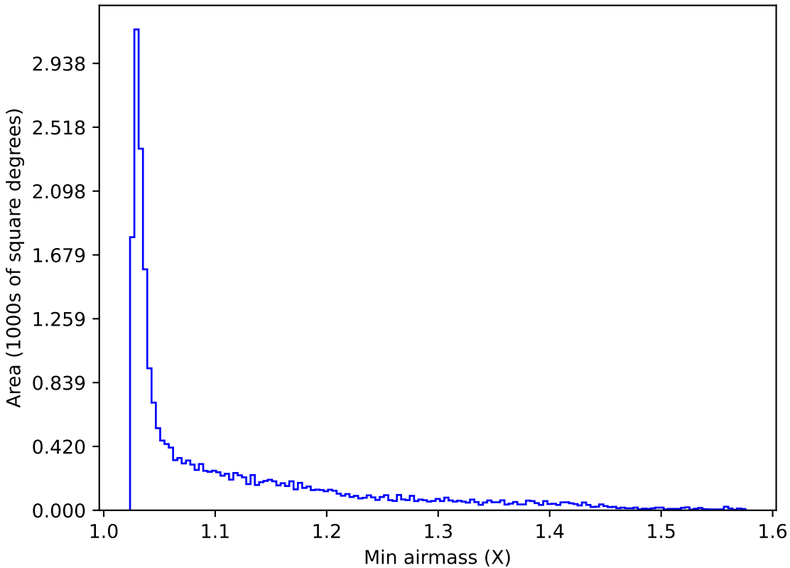
extra_ss_neo7_v3.4_10yrs All sky y band: Min airmass
