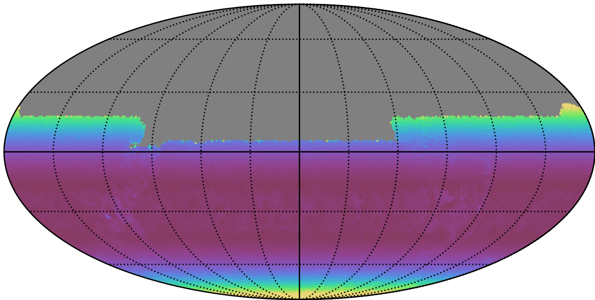
extra_ss_neo7_v3.4_10yrs All sky u band: Min airmass
