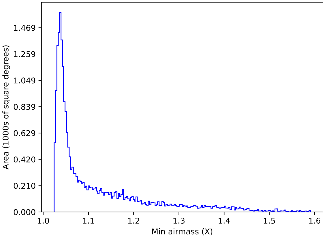
extra_ss_neo7_v3.4_10yrs All sky u band: Min airmass
