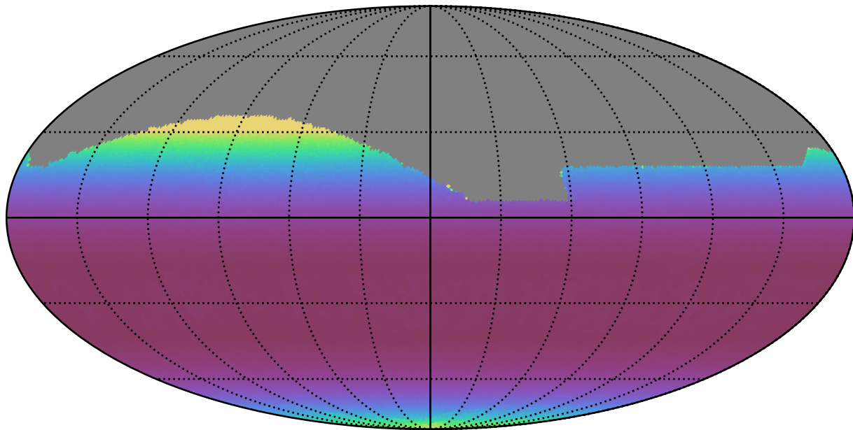
extra_ss_neo7_v3.4_10yrs All sky r band: Min airmass
