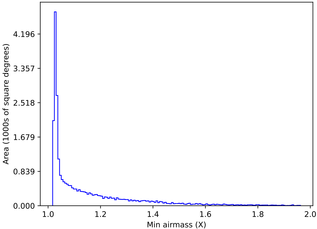
extra_ss_neo7_v3.4_10yrs All sky r band: Min airmass
