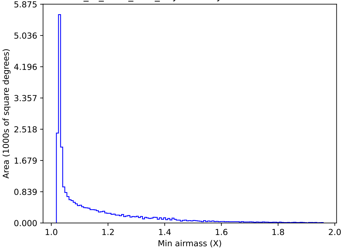
extra_ss_neo7_v3.4_10yrs All sky i band: Min airmass
