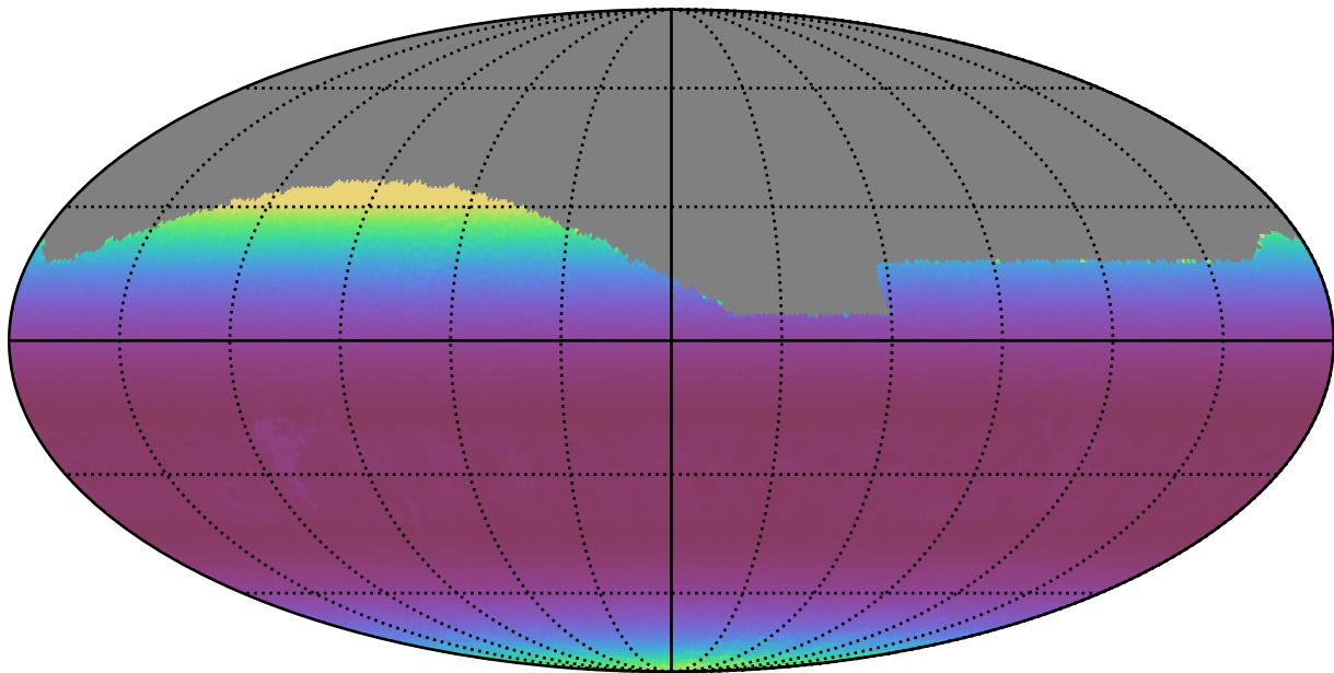
extra_ss_neo7_v3.4_10yrs All sky g band: Min airmass
