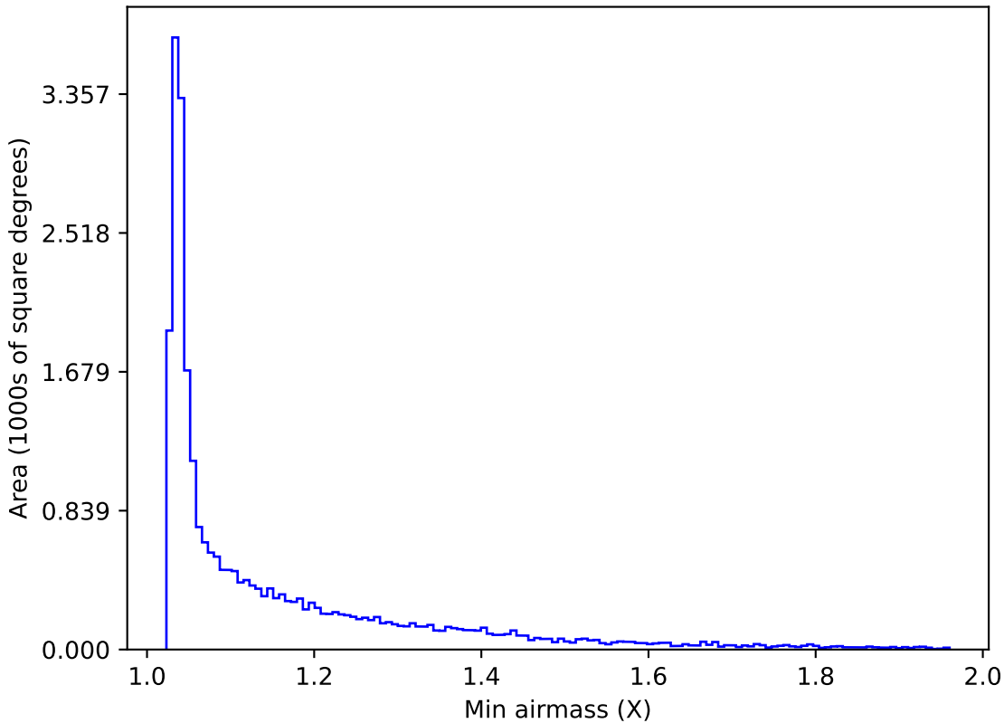
extra_ss_neo7_v3.4_10yrs All sky g band: Min airmass
