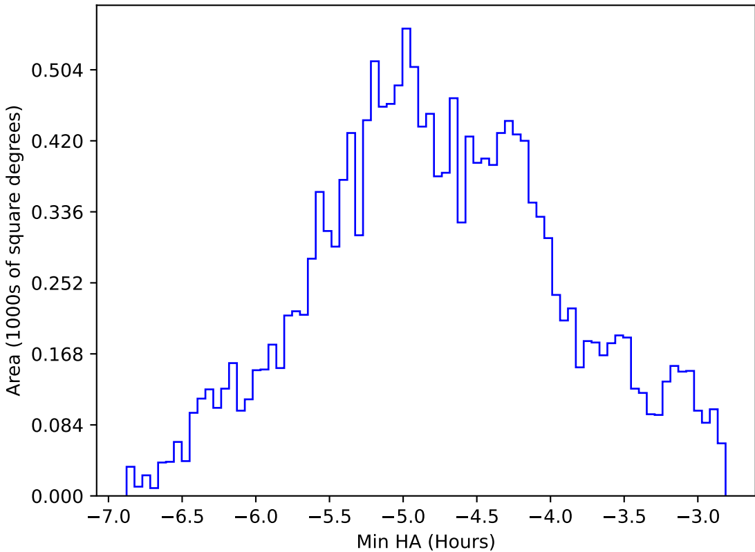
extra_ss_neo7_v3.4_10yrs WFD all bands: Min HA
