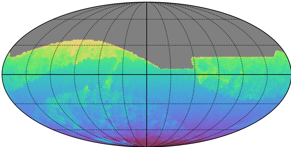
extra_ss_neo7_v3.4_10yrs All sky all bands: Min HA
