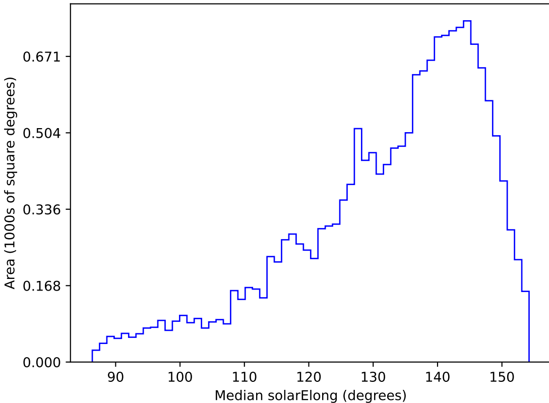
extra_ss_neo7_v3.4_10yrs WFD u band: Median solarElong
