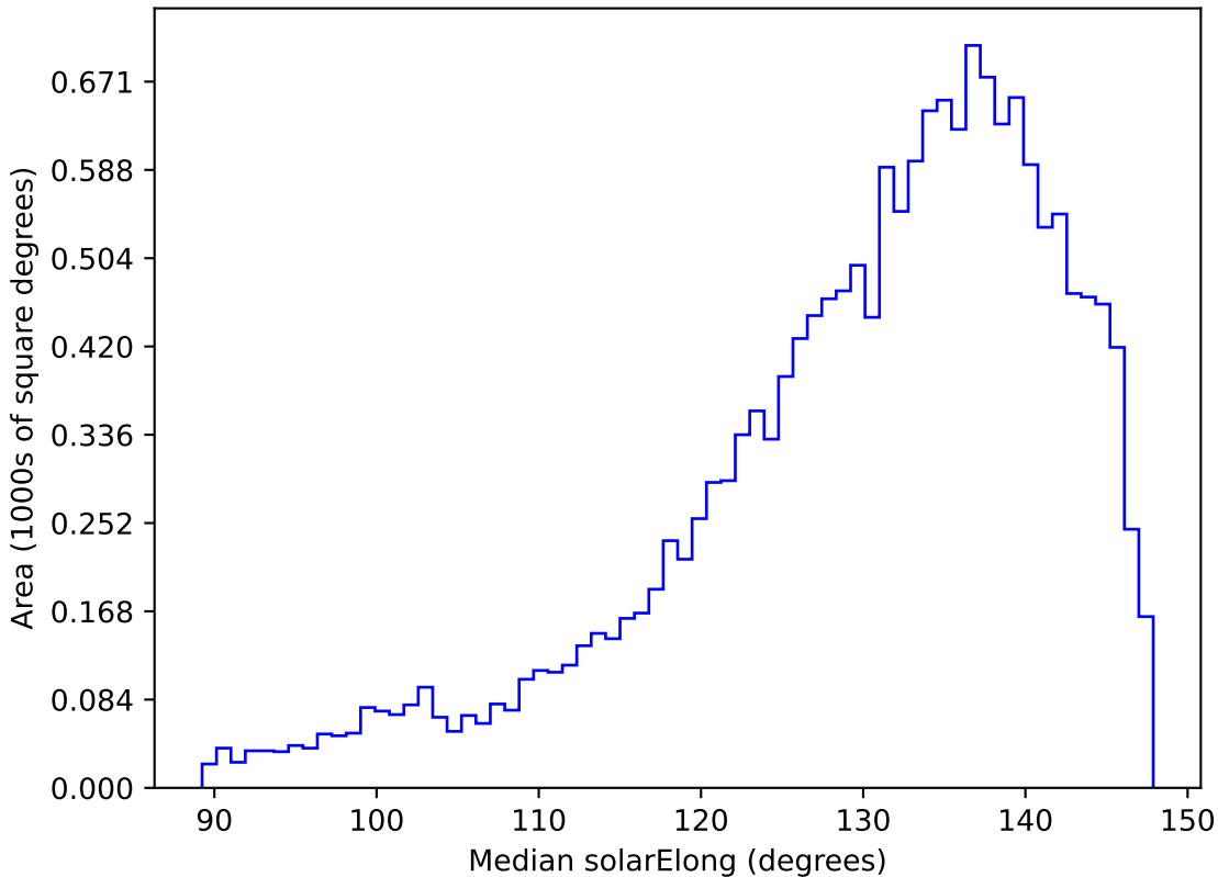
extra_ss_neo7_v3.4_10yrs WFD r band: Median solarElong
