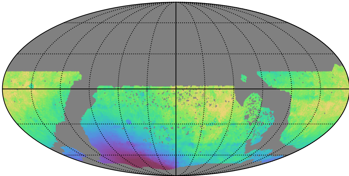
extra_ss_neo7_v3.4_10yrs WFD i band: Median solarElong
