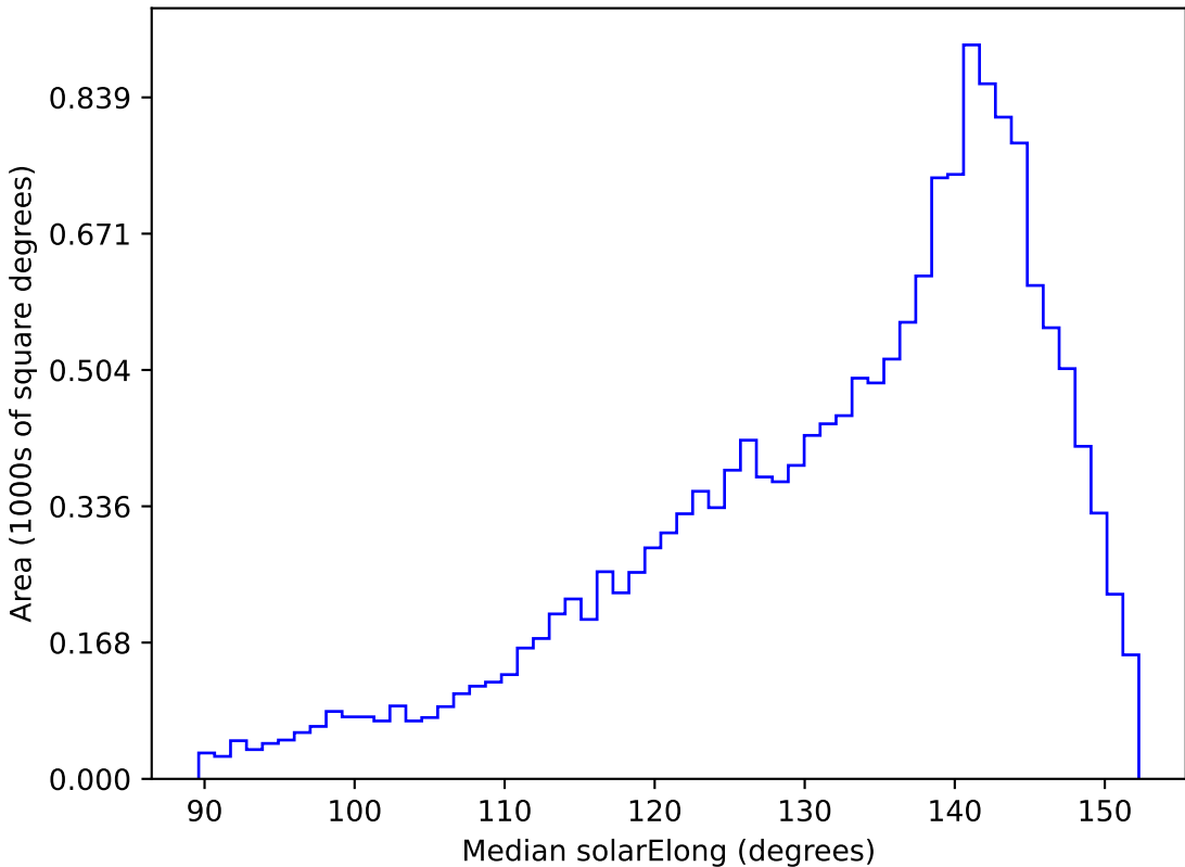
extra_ss_neo7_v3.4_10yrs WFD g band: Median solarElong
