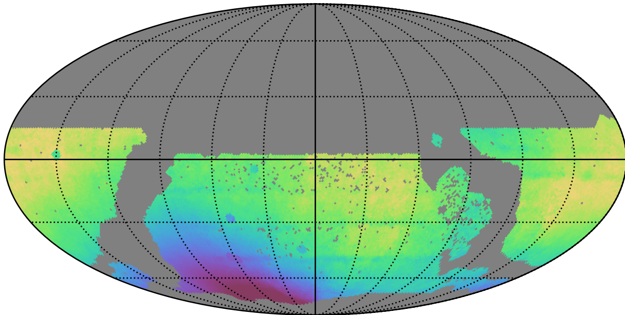
extra_ss_neo7_v3.4_10yrs WFD all bands: Median solarElong
