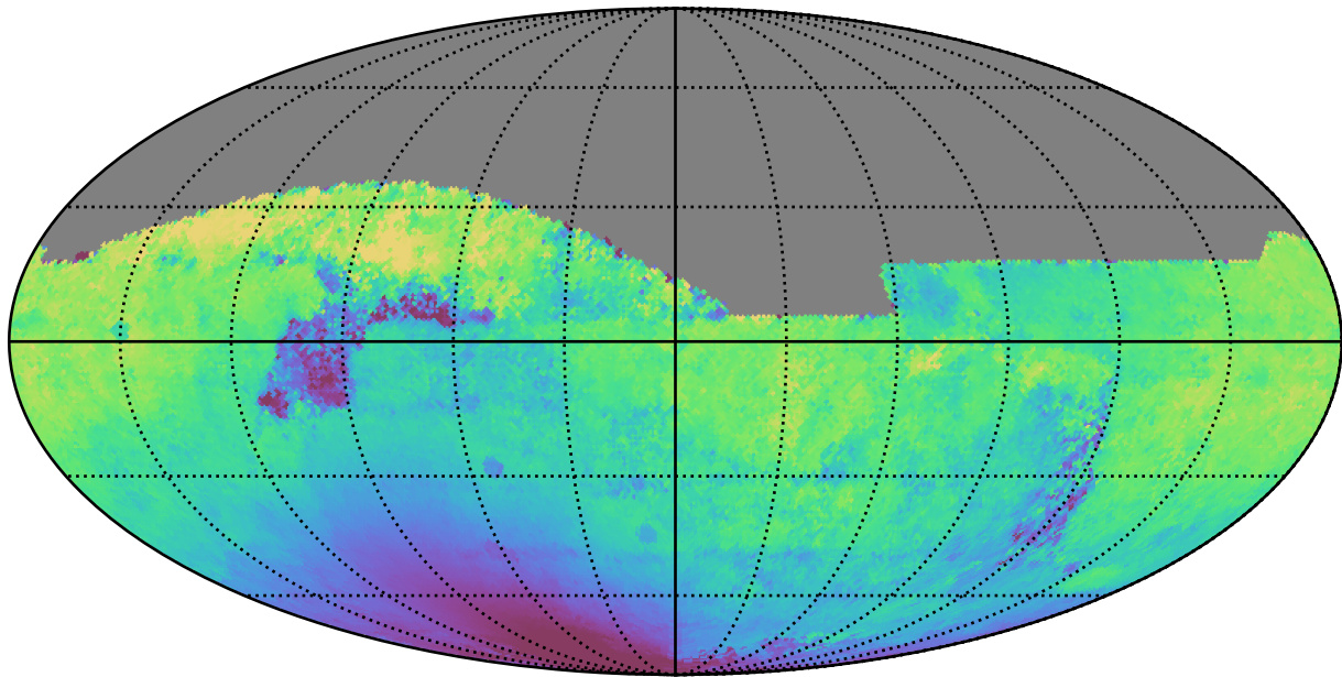
extra_ss_neo7_v3.4_10yrs All sky z band: Median solarElong
