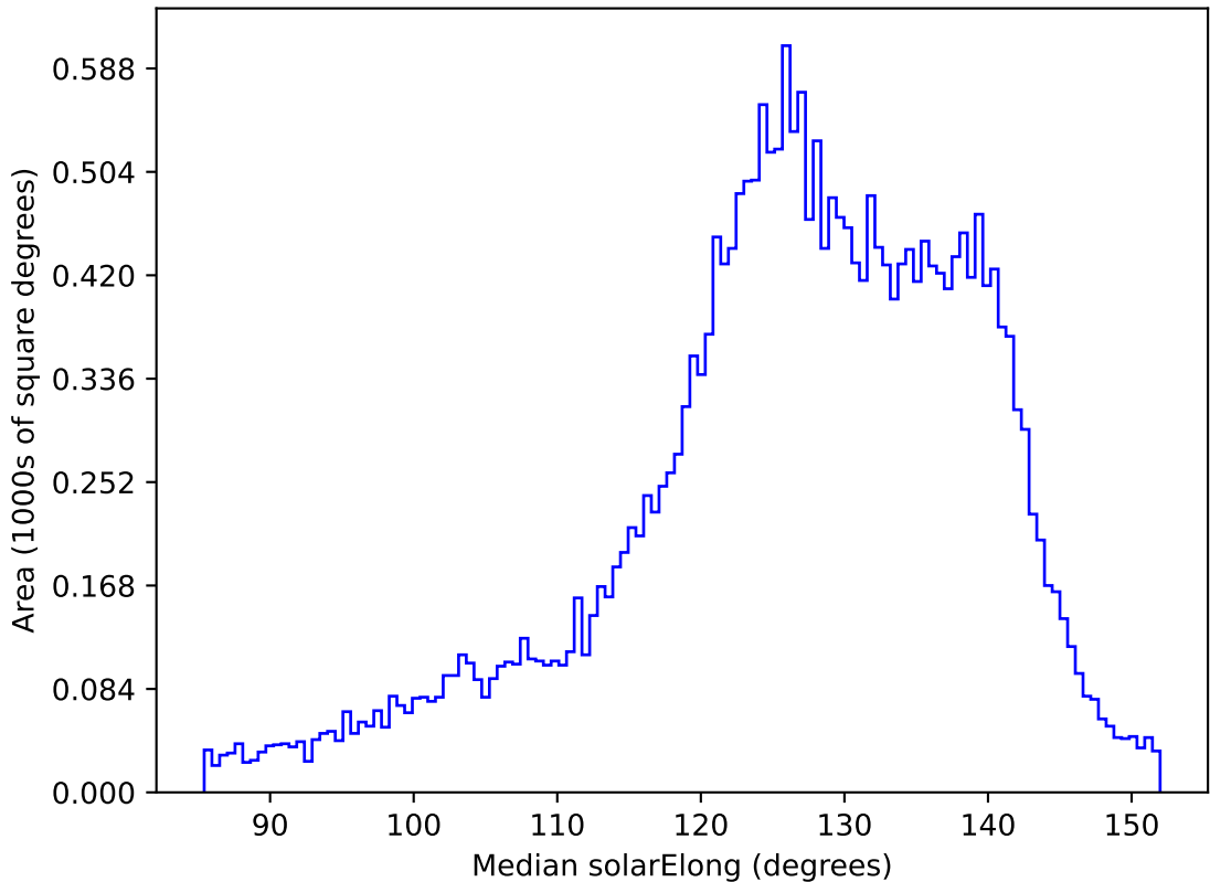
extra_ss_neo7_v3.4_10yrs All sky z band: Median solarElong
