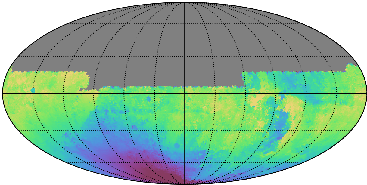
extra_ss_neo7_v3.4_10yrs All sky u band: Median solarElong
