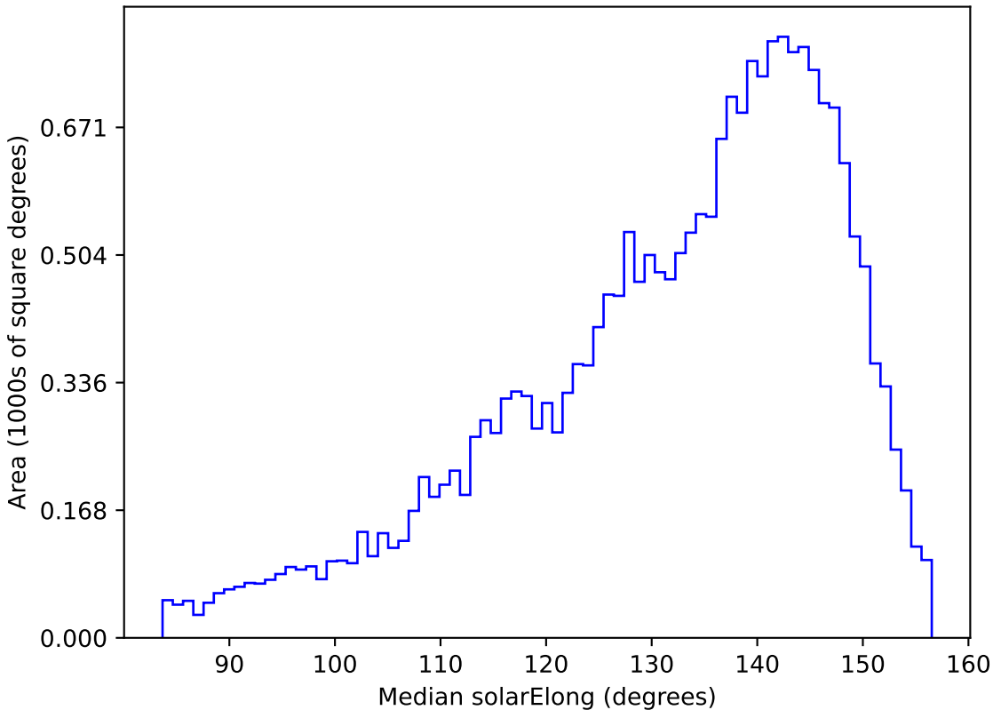
extra_ss_neo7_v3.4_10yrs All sky u band: Median solarElong
