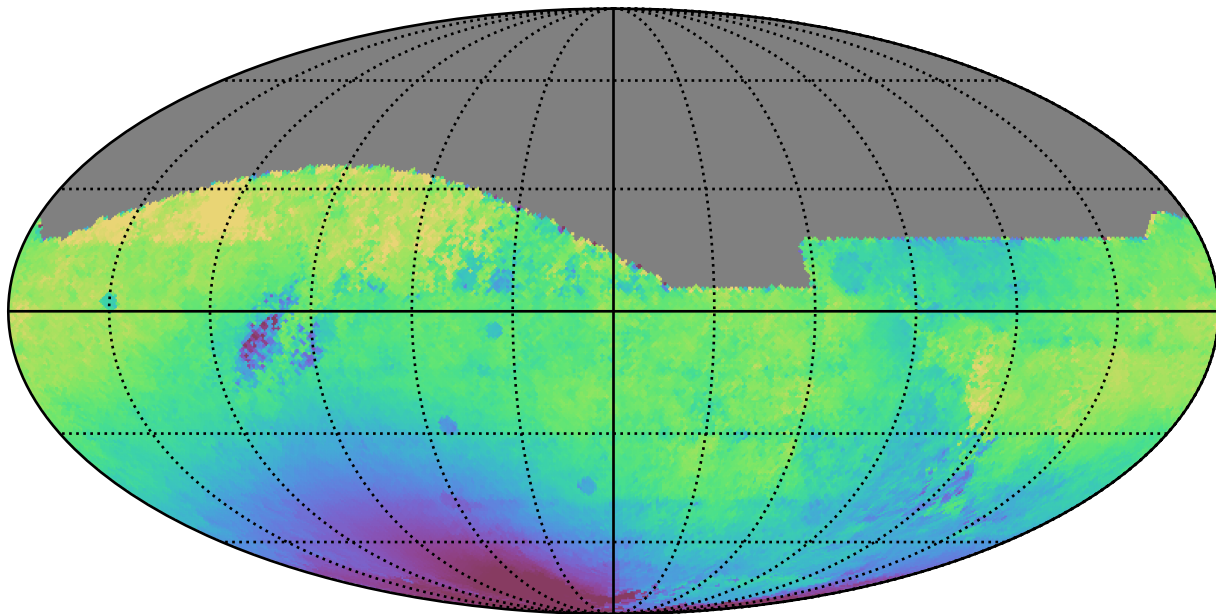
extra_ss_neo7_v3.4_10yrs All sky r band: Median solarElong
