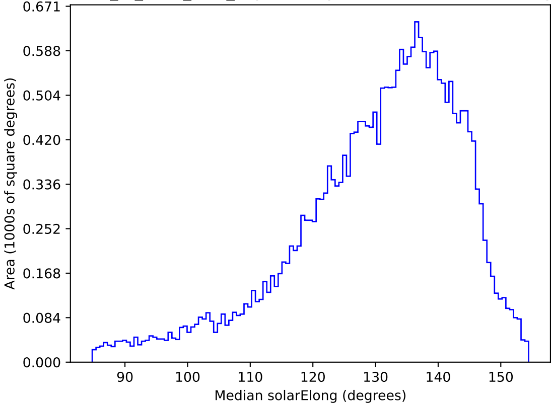
extra_ss_neo7_v3.4_10yrs All sky r band: Median solarElong
