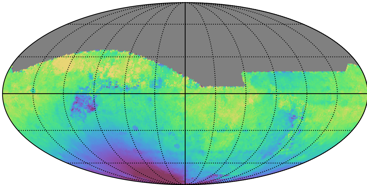
extra_ss_neo7_v3.4_10yrs All sky i band: Median solarElong
