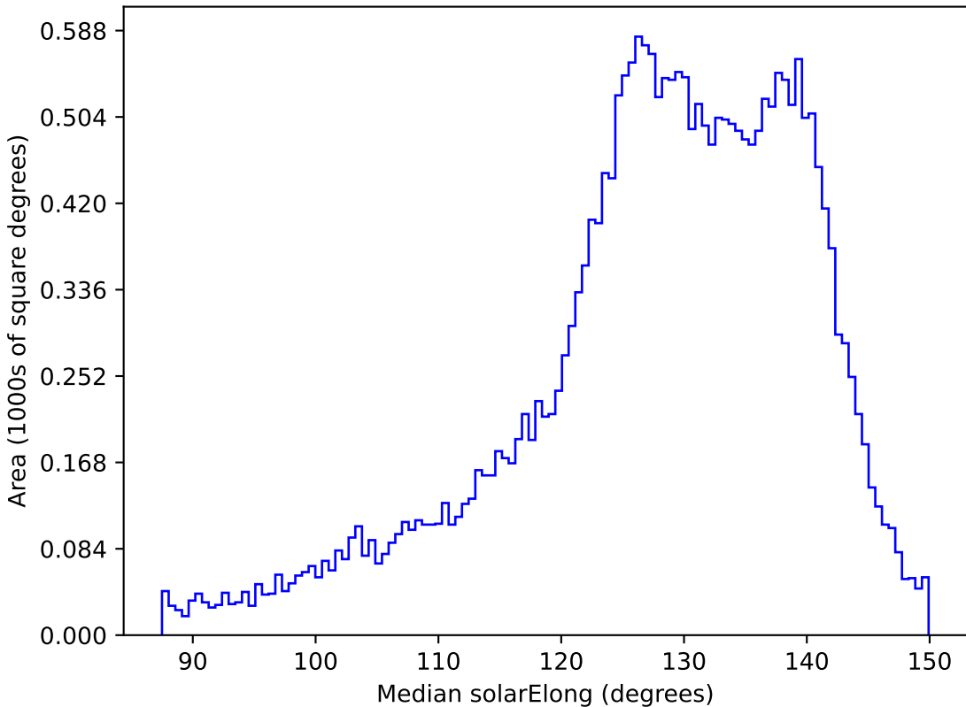
extra_ss_neo7_v3.4_10yrs All sky i band: Median solarElong
