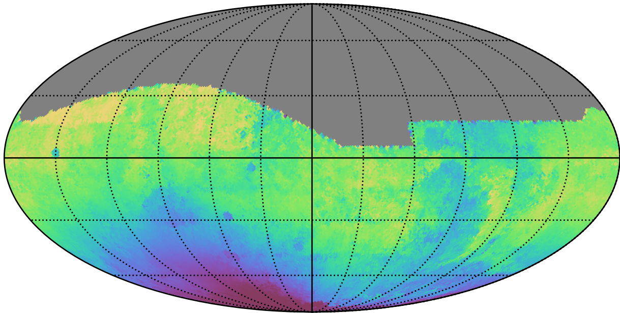
extra_ss_neo7_v3.4_10yrs All sky g band: Median solarElong
