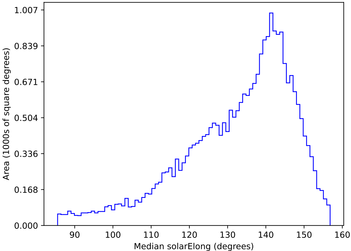
extra_ss_neo7_v3.4_10yrs All sky g band: Median solarElong
