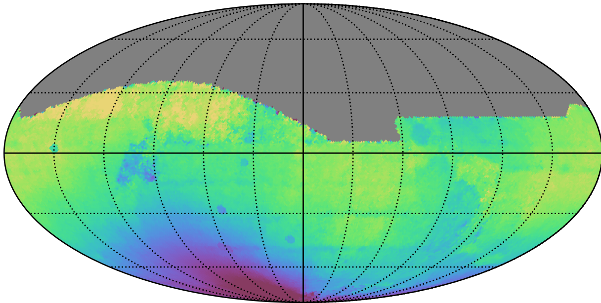
extra_ss_neo7_v3.4_10yrs All sky all bands: Median solarElong
