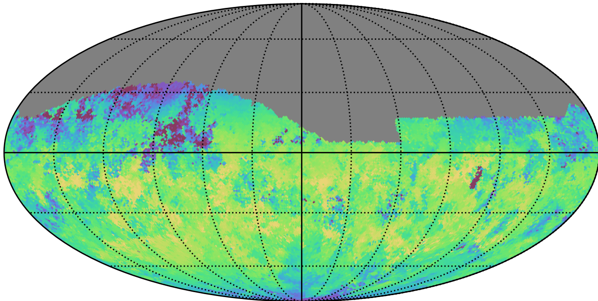
extra_ss_neo7_v3.4_10yrs Yr 1 z band: Median skyBrightness
