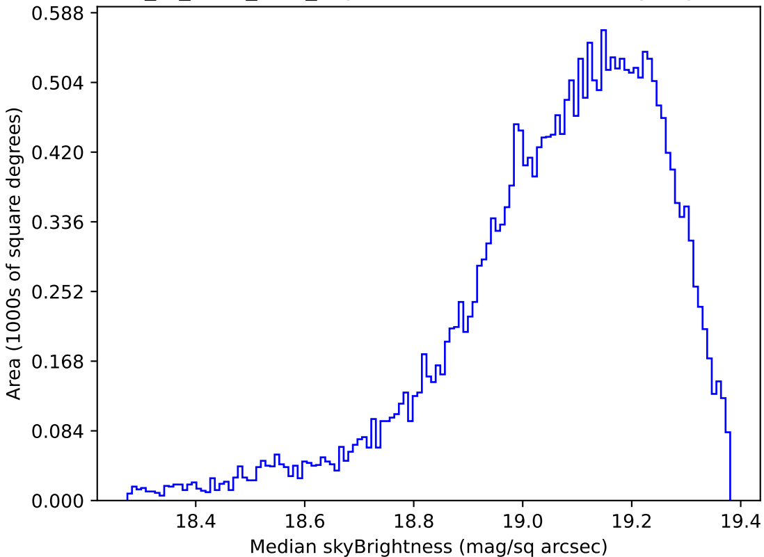
extra_ss_neo7_v3.4_10yrs Yr 1 z band: Median skyBrightness
