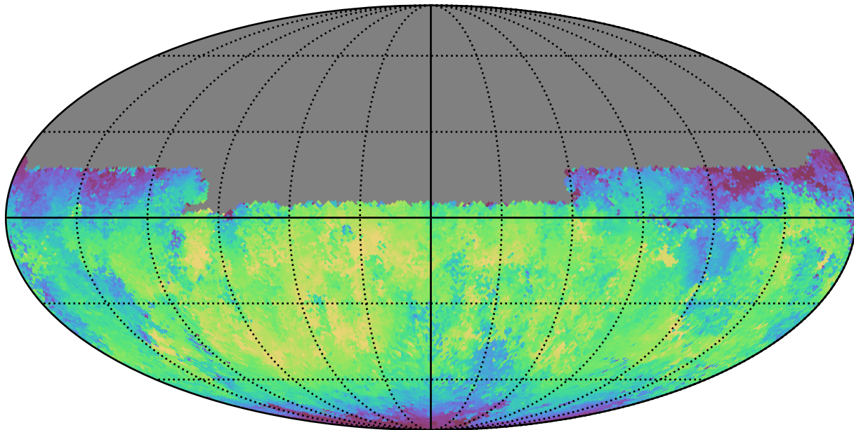
extra_ss_neo7_v3.4_10yrs Yr 1 y band: Median skyBrightness
