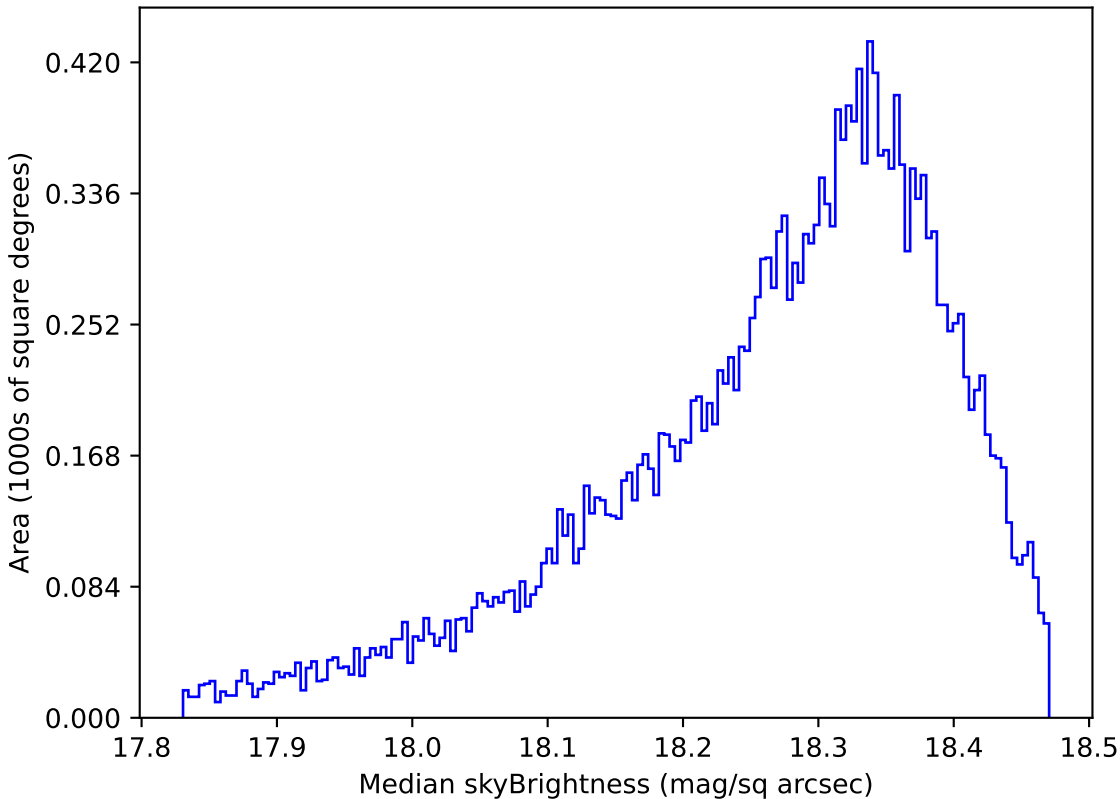
extra_ss_neo7_v3.4_10yrs Yr 1 y band: Median skyBrightness
