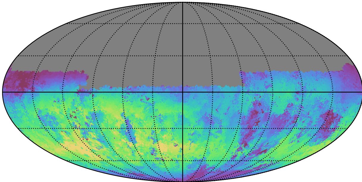
extra_ss_neo7_v3.4_10yrs Yr 1 u band: Median skyBrightness
