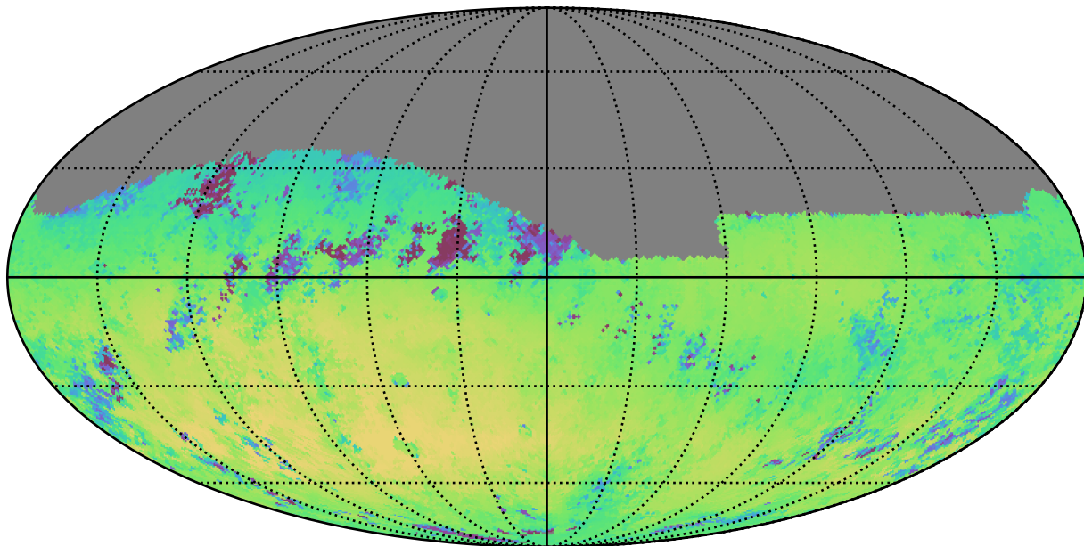
extra_ss_neo7_v3.4_10yrs Yr 1 r band: Median skyBrightness
