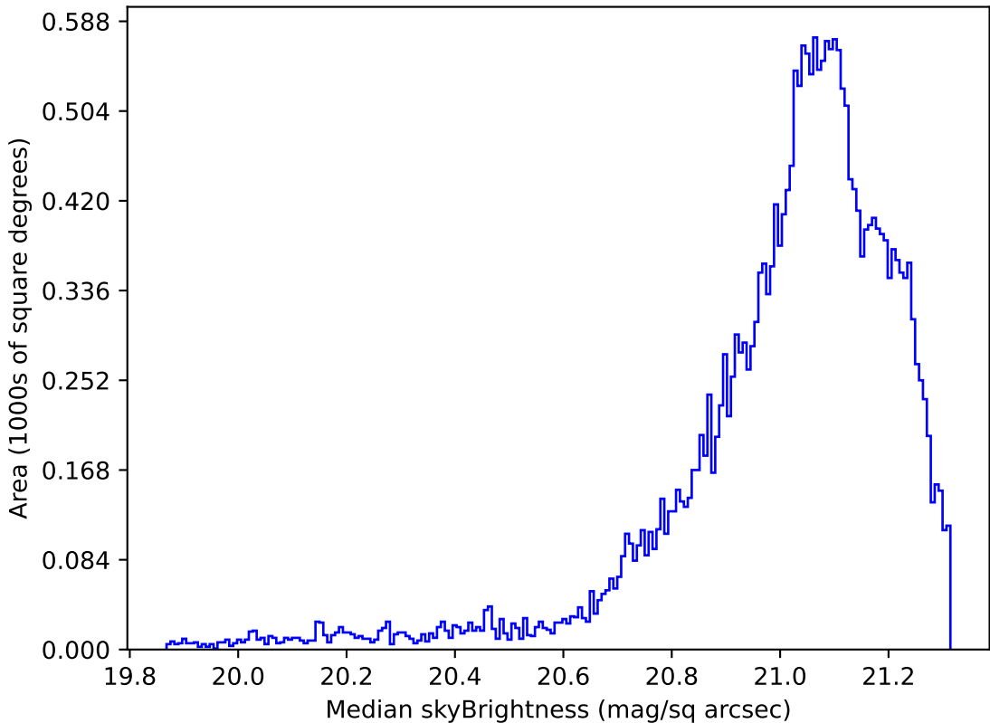
extra_ss_neo7_v3.4_10yrs Yr 1 r band: Median skyBrightness
