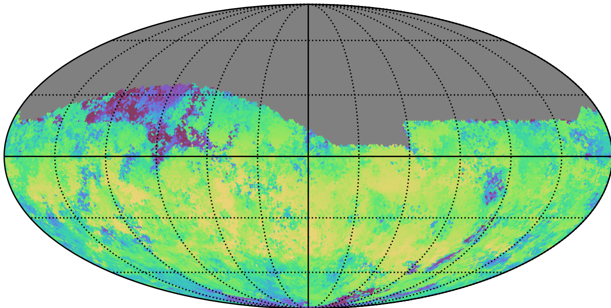
extra_ss_neo7_v3.4_10yrs Yr 1 i band: Median skyBrightness
