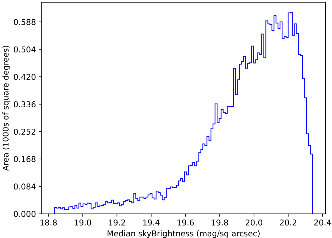
extra_ss_neo7_v3.4_10yrs Yr 1 i band: Median skyBrightness
