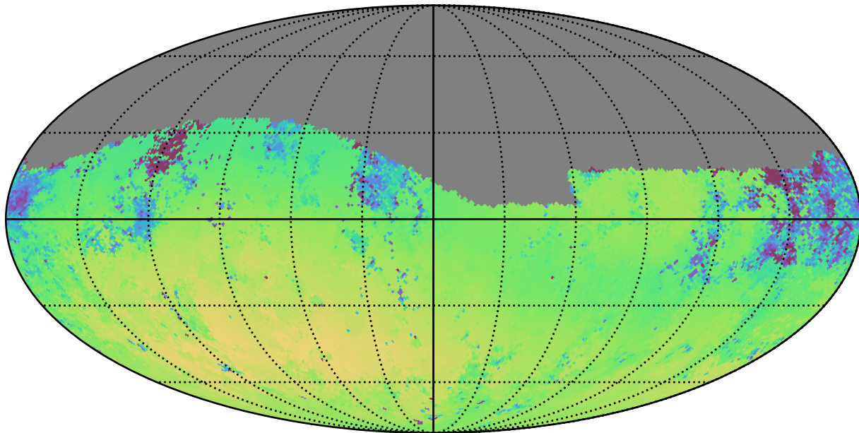
extra_ss_neo7_v3.4_10yrs Yr 1 g band: Median skyBrightness
