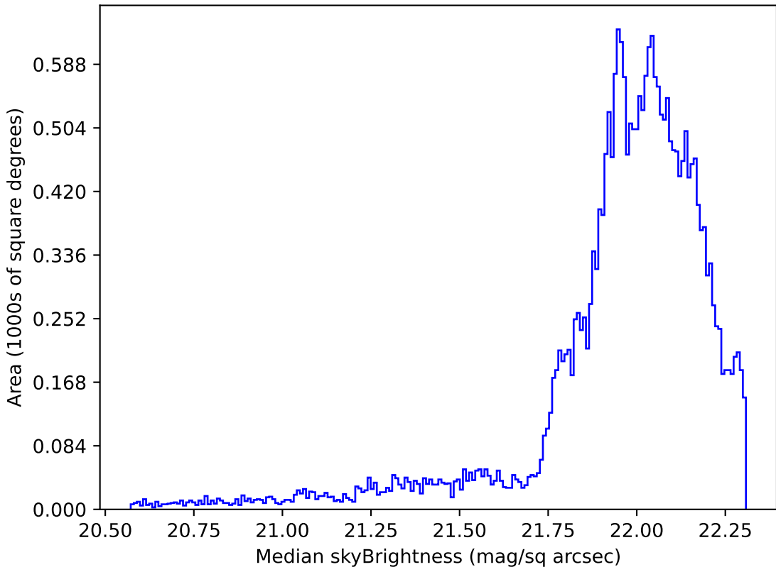
extra_ss_neo7_v3.4_10yrs Yr 1 g band: Median skyBrightness
