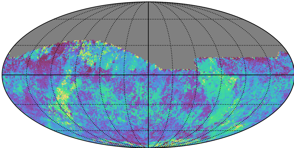
extra_ss_neo7_v3.4_10yrs Yr 1 all bands: Median skyBrightness
