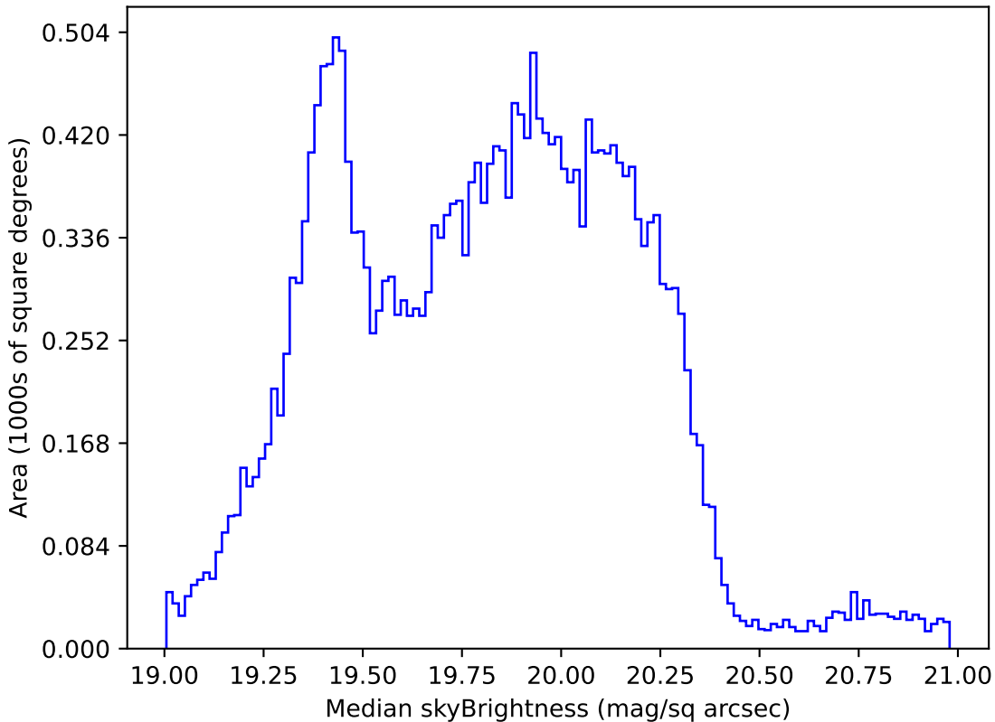
extra_ss_neo7_v3.4_10yrs Yr 1 all bands: Median skyBrightness
