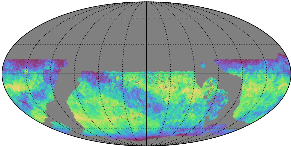
extra_ss_neo7_v3.4_10yrs WFD z band: Median skyBrightness
