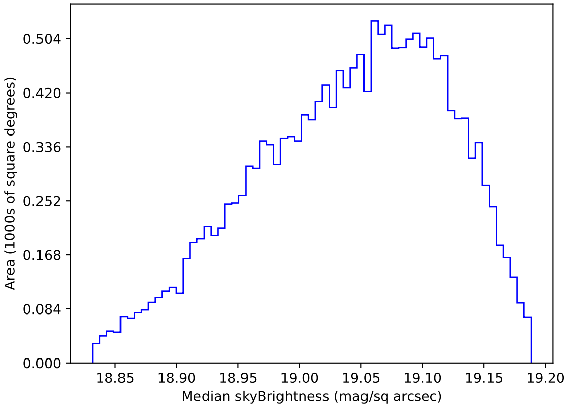
extra_ss_neo7_v3.4_10yrs WFD z band: Median skyBrightness
