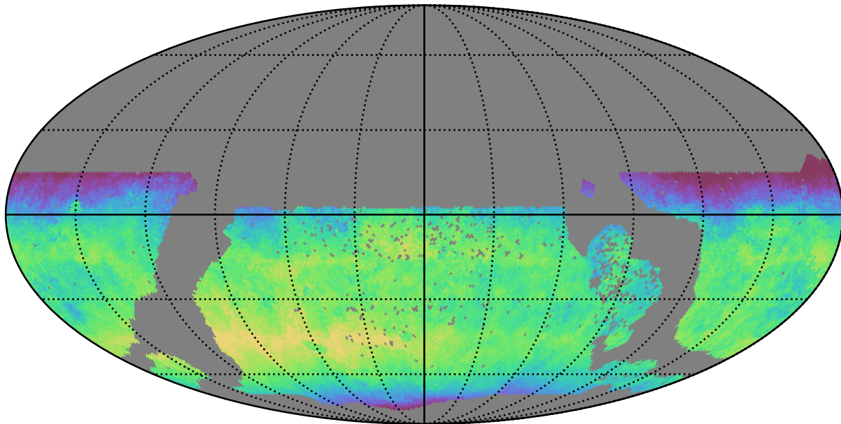
extra_ss_neo7_v3.4_10yrs WFD y band: Median skyBrightness
