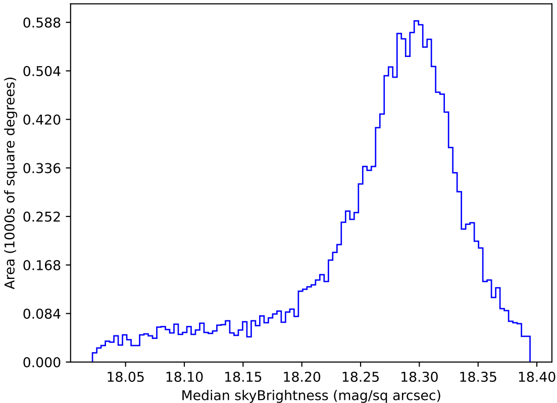
extra_ss_neo7_v3.4_10yrs WFD y band: Median skyBrightness
