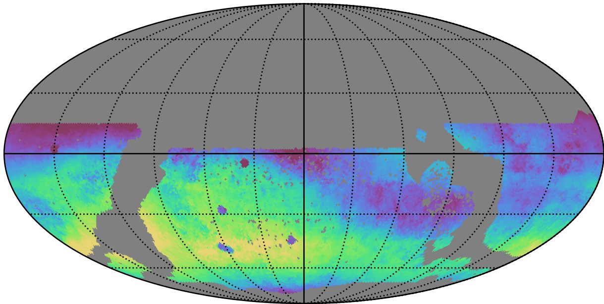
extra_ss_neo7_v3.4_10yrs WFD r band: Median skyBrightness
